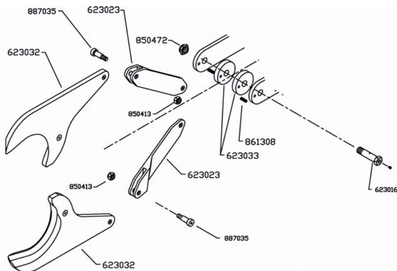
Figure 1 MODEL AHC – BLADE REPLACEMENT
