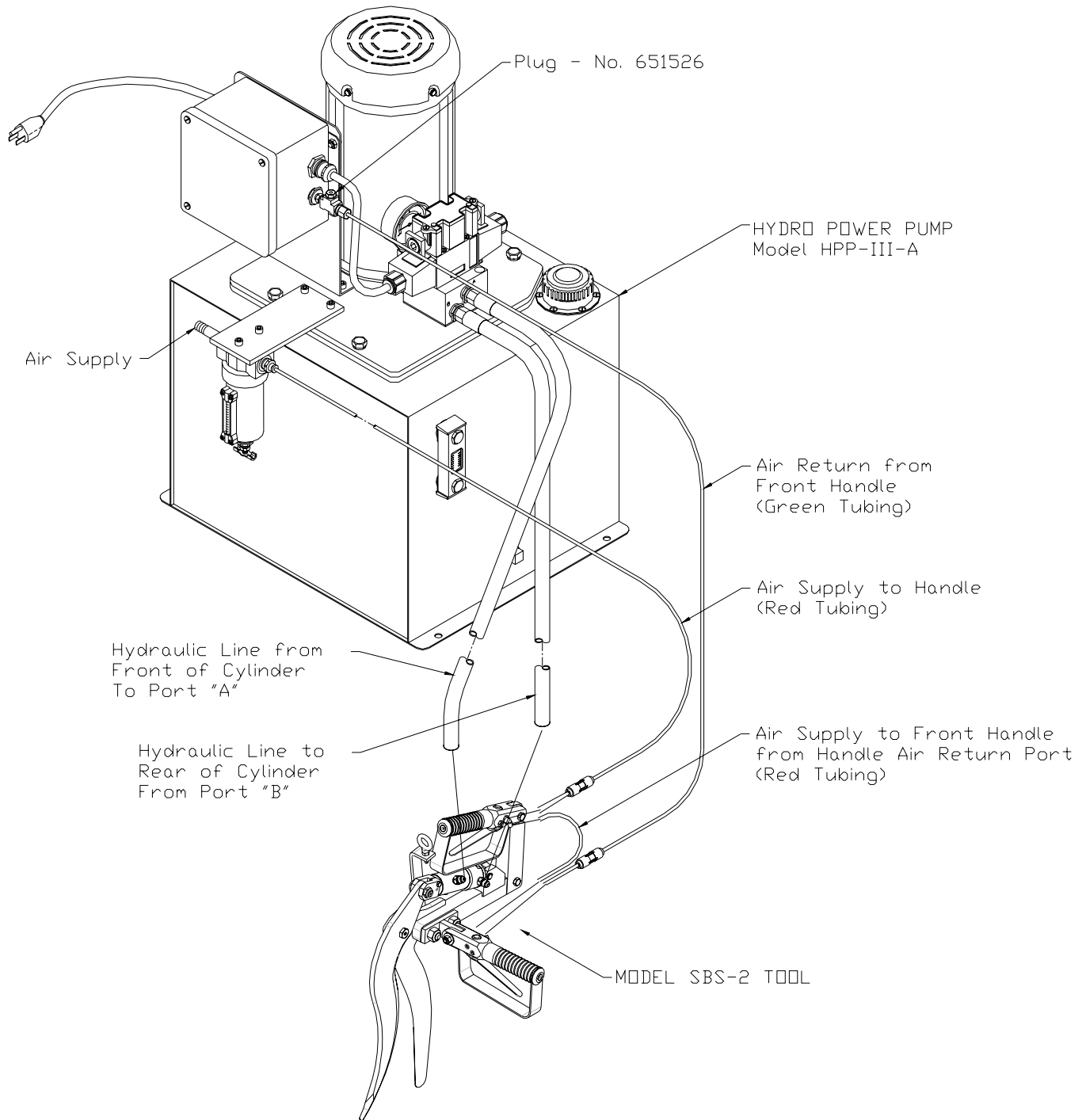
Figure 6 SBS-2 TUBING DIAGRAM – WITHOUT ANTI-TIE DOWN
