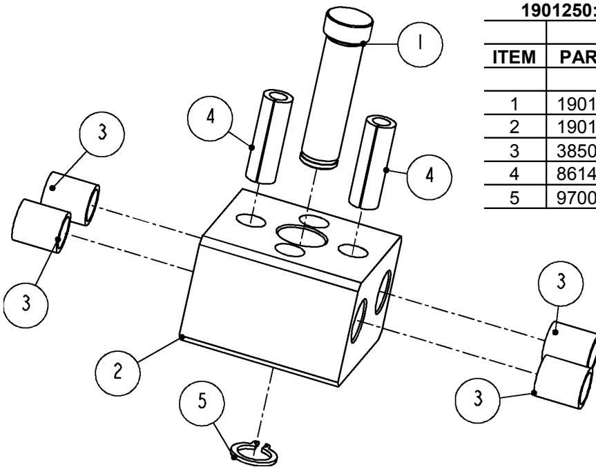
Figure 9 1901250: COUNTER BALANCE ASS'Y
