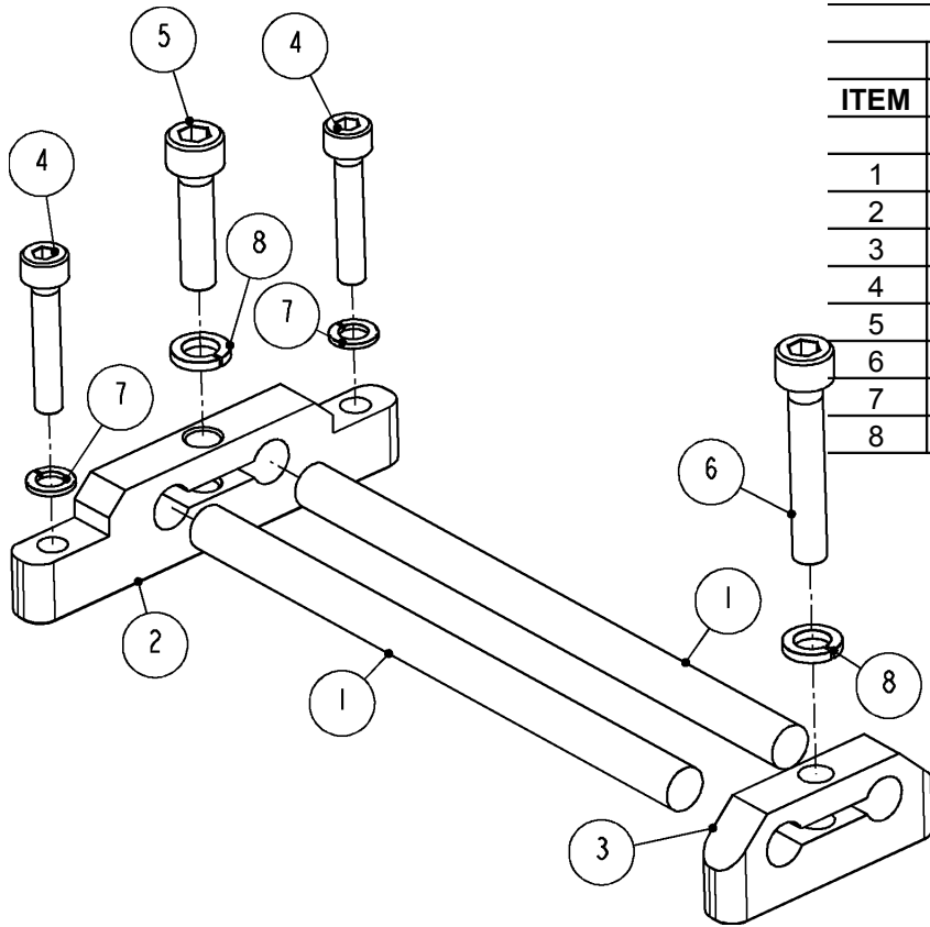
Figure 10 1901430: GUIDE ASSEMBLY
