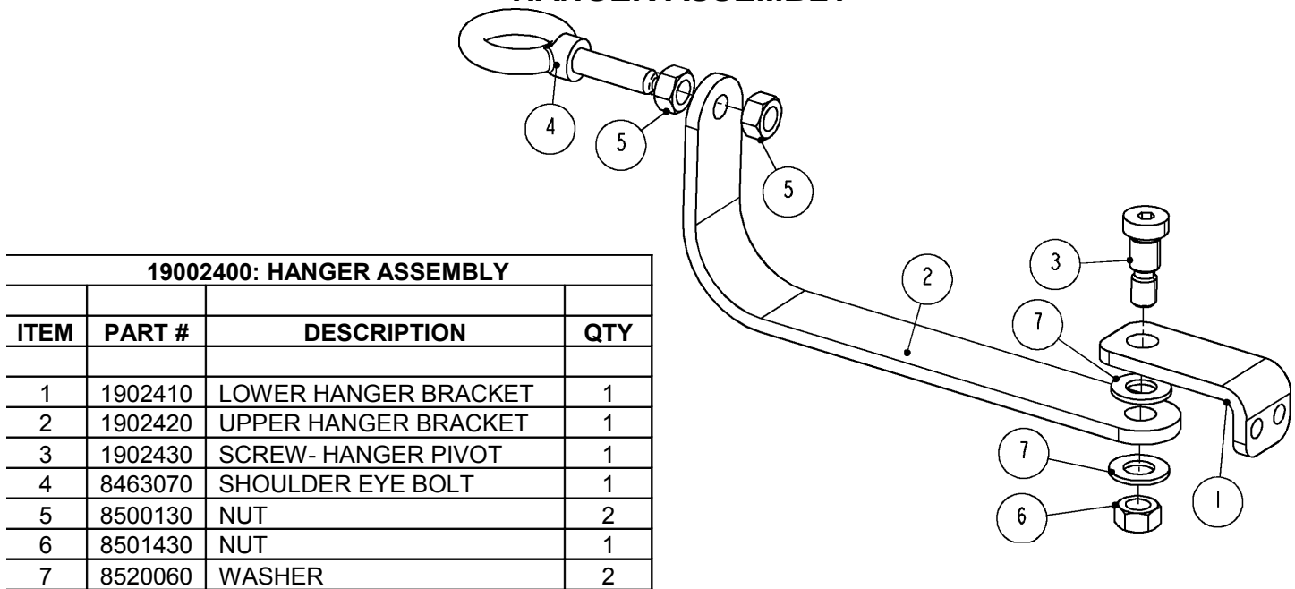
Figure 19 1902400: HANGER ASSEMBLY
