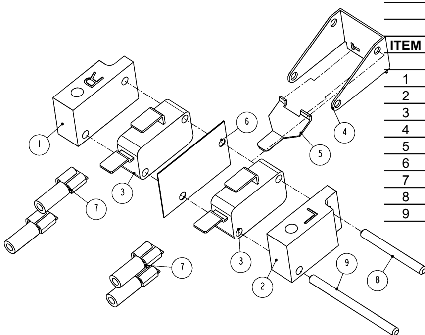
Figure 17 1902600: SWITCH ASSEMBLY
