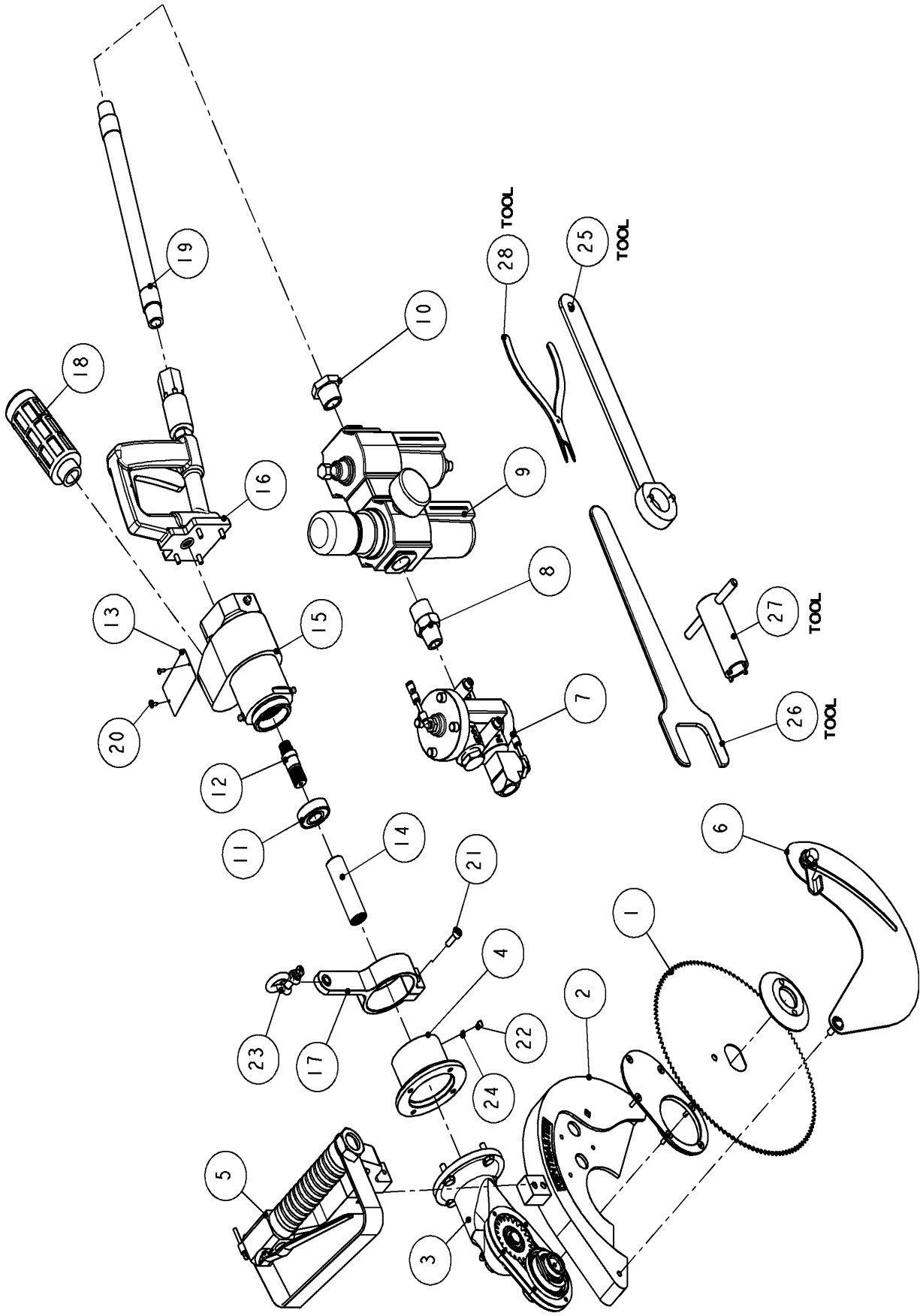
Figure 2 MODEL "77" – MAIN ASSEMBLY
